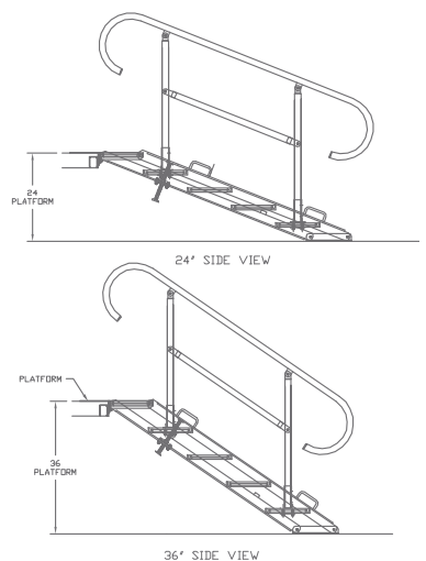
24 inch - 36 inch Adjustable Height Stair Unit
