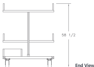
End View
